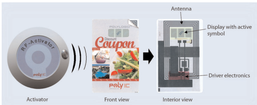
Fig. 2. A radio-activated display consists of a thin flexible display (centre top and top right) with receiver circuit (right) and an activation unit (left)
